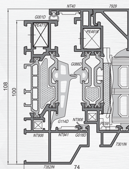
Frame and window sash
