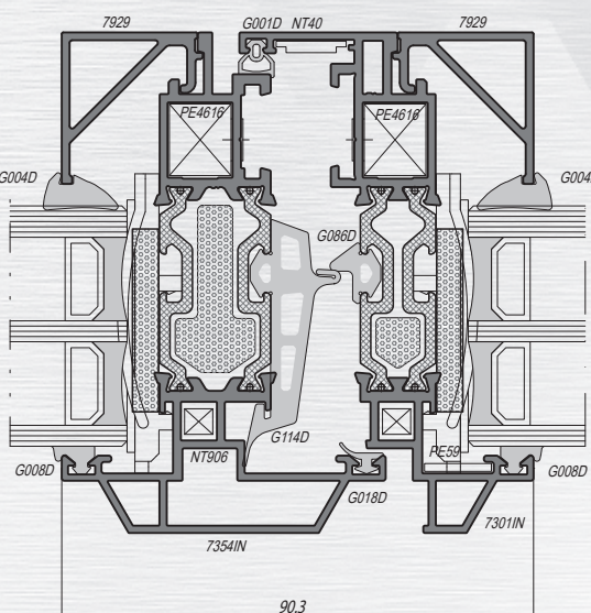
Window sash with floating mullion
